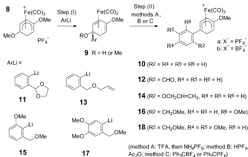
Scheme 1. Preparation of (1-arylcyclohexadienyl)iron complexes.
