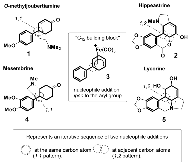
Figure 1. Examples of alkaloid target molecules to illustrate a general organoiron-mediated approach that makes multiple use of the metal: a “C 12 building block” based on an arylcyclohexadienyl complex corresponds to the central pair of six-membered rings in structures of this type (the requirements for iterative [9] metal-mediated bond formation are indicated as 1,1 or 1,2 [6,7] by the dashed circles).
