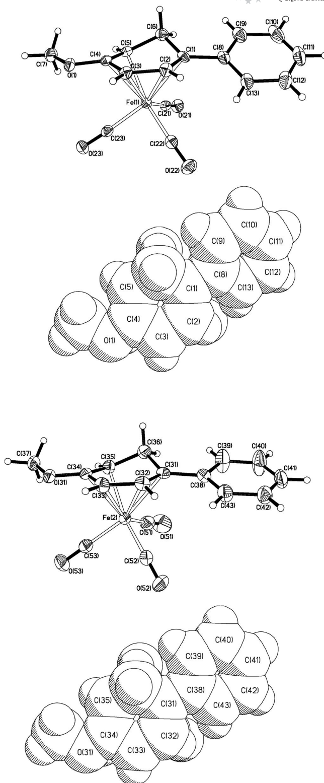
Figure 3. ORTEP and space-filling representations of molecules 1 (top) and 2 (bottom) in the X-ray structure of tricarbonyl[(1-5- \eta )-4-methoxy-1-phenylcyclohexadienyl]iron hexafluorophosphate ( 10 ).
