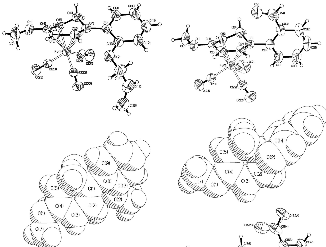
Figure 4. ORTEP and space-filling representations of the X-ray structure of tricarbonyl[(1-5-η)-1-(2'-allyloxyphenyl)-4-methoxycyclohexadienyl]iron hexafluorophosphate ( 14 ).
