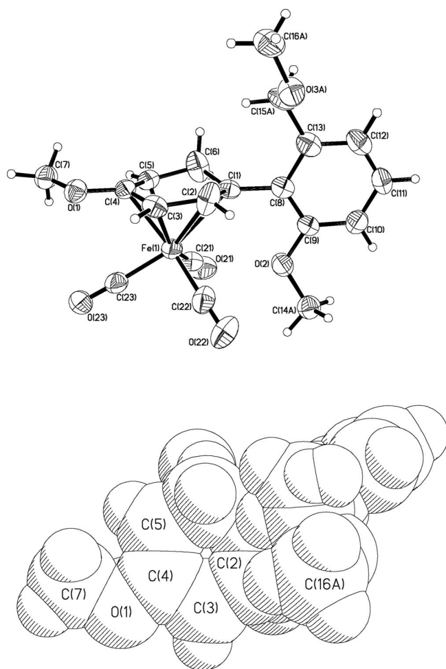
Figure 6. ORTEP and space-filling representations of the X-ray structure of tricarbonyl[(1-5- \eta )-1-(2'-methoxymethyl-6'-methoxyphenyl)-4-methoxycyclohexadienyl]iron hexafluorophosphate ( 16 ). For clarity, only the major conformers of disordered methoxy groups are shown.
