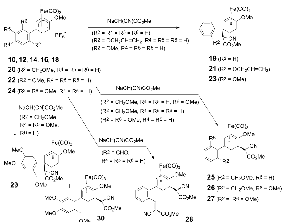
Scheme 2. Nucleophile addition to (1-arylcyclohexadienyl)iron complexes.
