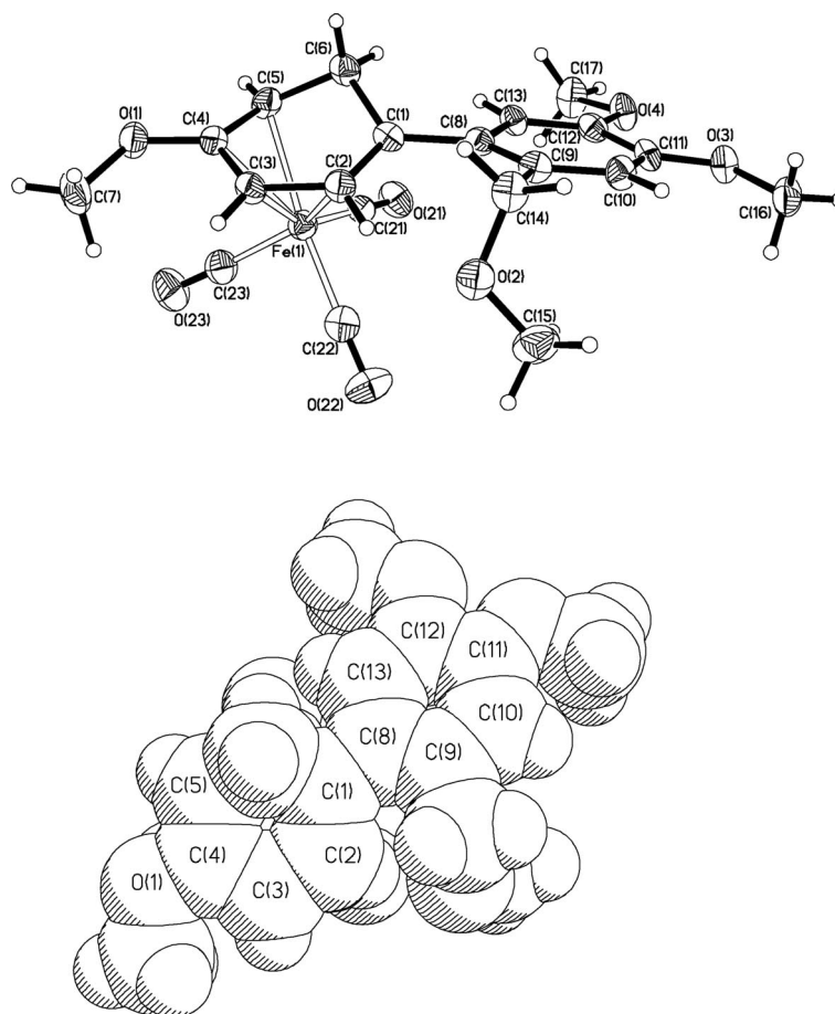
Figure 7. ORTEP and space-filling representations of the X-ray structure of tricarbonyl{(1-5- \eta )-1-[4',5'-dimethoxy-2'-(methoxymethyl)-phenyl]-4-methoxycyclohexadienyl}iron hexafluorophosphate ( 18 ).
